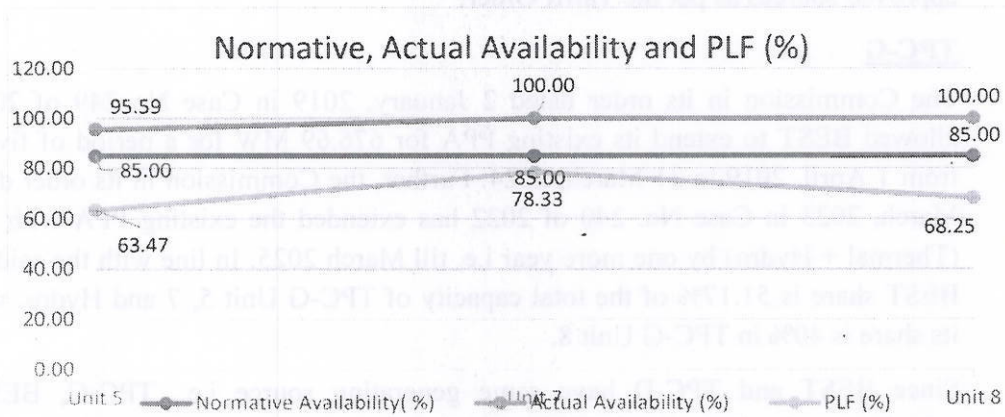
Figure 2: PAF and PLF of TPC Generating Units
